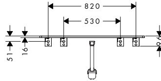
Xelu Q 1360/550 54098XX0
