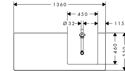
Xelu Q 1360/550 54098XX0
